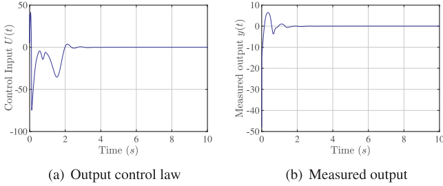
Fig. 4. Evolution of the control law and the measured output.
