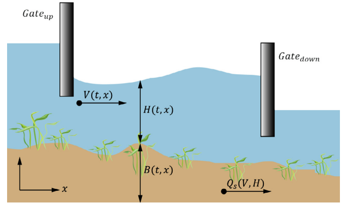
Fig. 1. A sketch of the channel.
