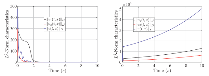
(a) Backstepping design.
