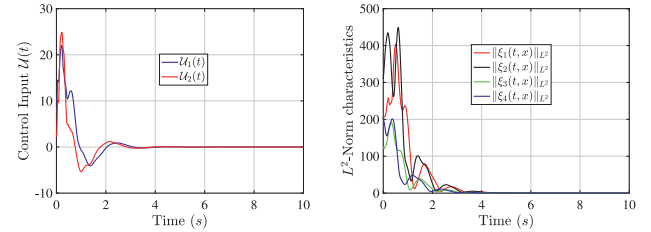
Fig. 8. Evolution in time of the control input U(t) and the norm of the characteristic solutions.
